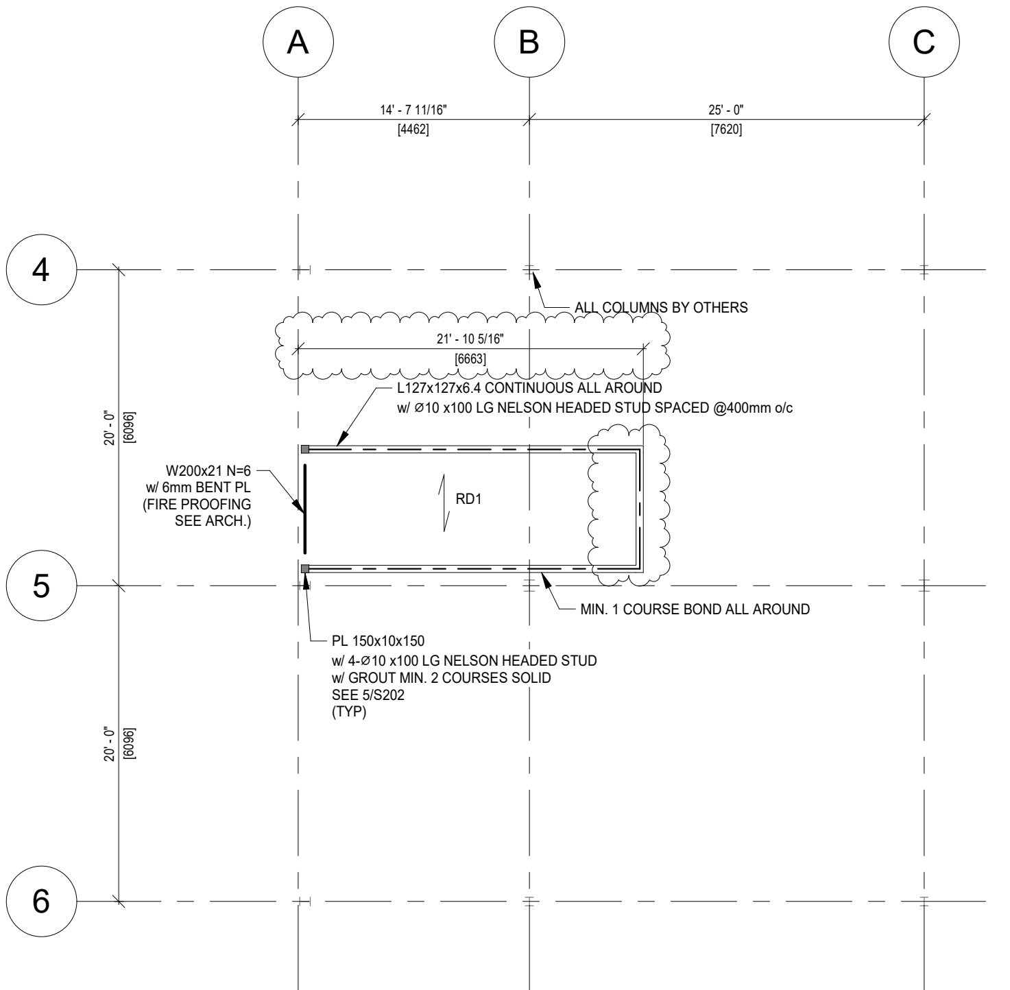
3 ROOF OF STAIRWELL B S202 1 : 100 NOTE: SEE ARCH. DRAWING FOR TOP ELEVATION
