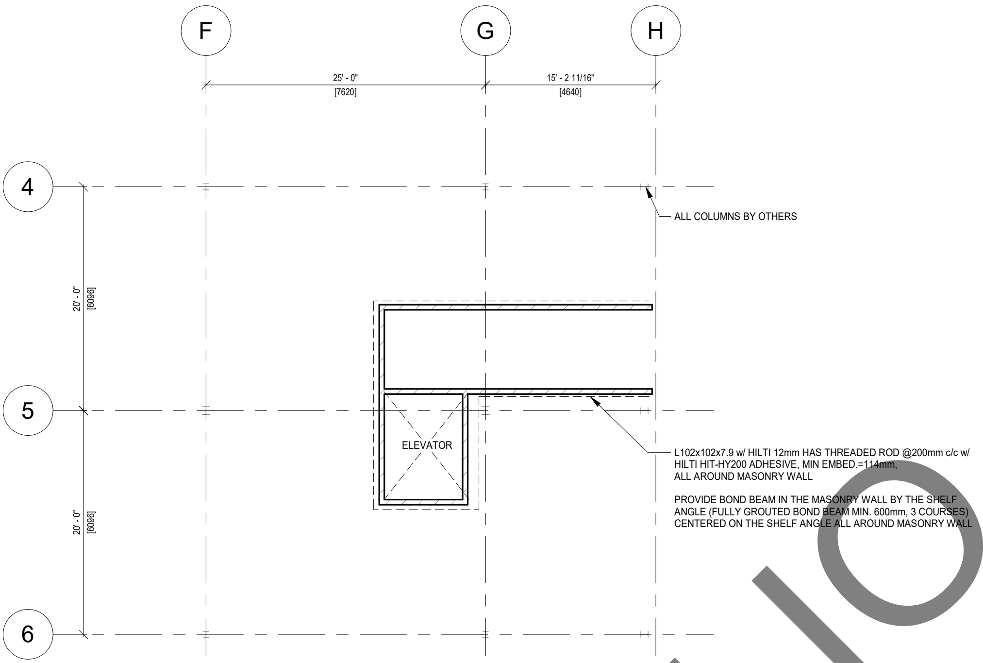
2 2ND FLOOR LEVEL - STAIRWELL A AND ELEVATOR S202 1 : 100
